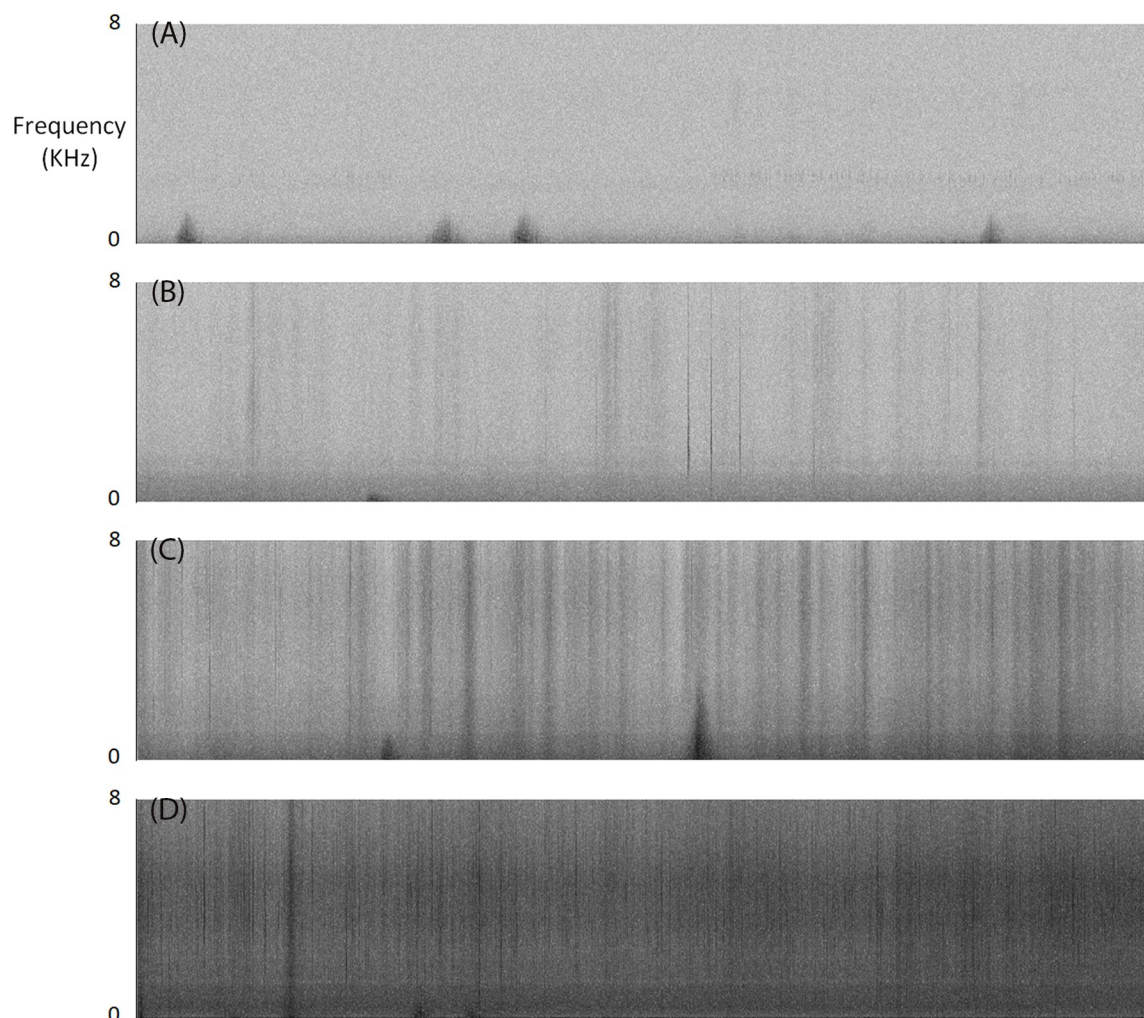
Fig 2. Spectrograms of recordings (one-hour duration) showing the influence of weather conditions on spectrogram clarity: (A) calm conditions with 0% spectrogram containing ambient noise, inclement weather score (IWS) = 0; (B) wind and rain causing ambient noise in 1–20% of spectrogram, IWS = 1; (C) wind and rain causing high levels of ambient noise in 21–50% of spectrogram, IWS = 2; and (D) wind and rain causing high levels of ambient noise in >50% of spectrogram, IWS = 3.
