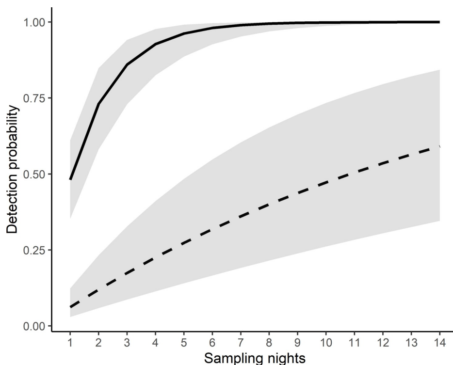
Fig 6. The relationship between the probability of detecting Yellow-bellied Glider vocalisations and the number of sampling nights with no inclement weather (mean score of 0; solid line) and frequent inclement weather (mean score of 3; dashed line). 95% confidence intervals are shaded grey.
