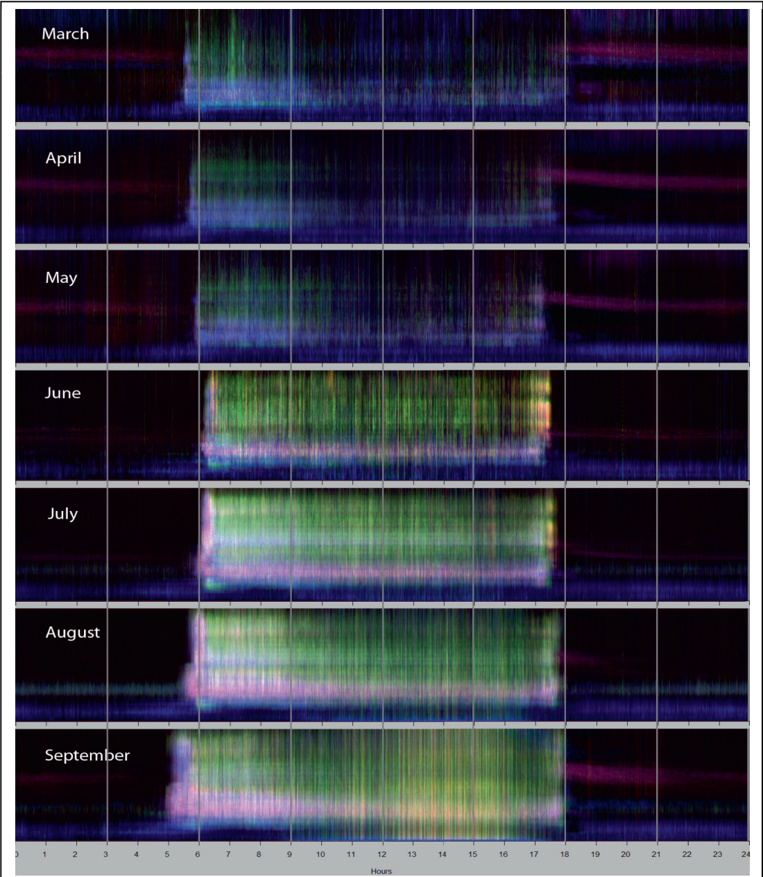
Figure 4: Monthly averaged spectrograms derived from the months March to September, 2013.
