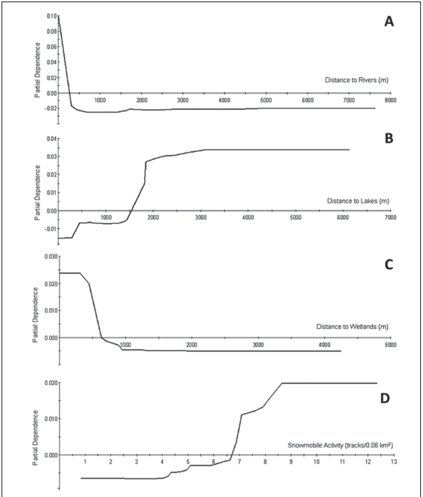
Figure 6. One predictor dependence for the top four environmental variables displaying their acoustic–environmental relationships with snowmobile noise in the Kenai National Wildlife Refuge (December 2011–April 2012): (A) distance to rivers, (B) distance to lakes, (C) distance to wetlands, and (D) snowmobile activity.
