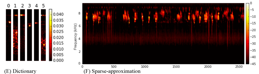
Figure 3 Over-complete Dictionaries (A), (C), (E) and sparse-approximations of original spectrogram (B), (D), (F) for Primary Forest site dawn chorus for Mini-batch gradient learning, Gabor Field Dictionary and SI- PLCA2D Component Dictionary.
