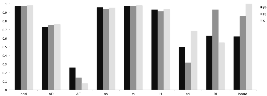
Figure 2 Bar plots of indices values for the three study sites. Plots show indices values for 10 min of dawn chorus. Values for AD, ACI and BI are scaled in the ranges 0:3, 1800:1900 and 0:12 respectively. Point count ‘heard’ data values for each site are given in the end column for comparison.
