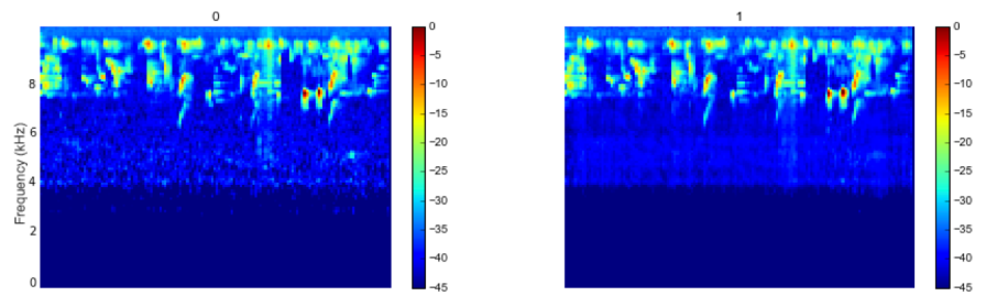
(A) S Original Spectrum ( S = 5.1797 )
