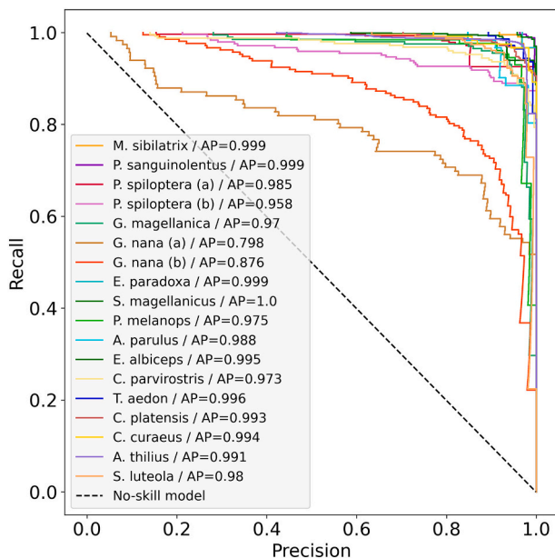
Fig. 5. Predictive performance of 18 classes according to precision-recall curves and AP per class.
