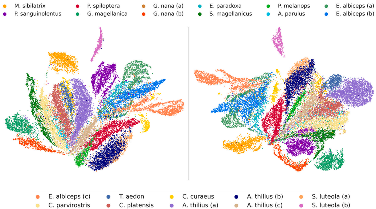
Fig. 4. UMAP visualization from the hyper-vectors of acoustic features, corresponding to the 22,243 samples labeled as presence. Left: UMAP fed with STFT features. Right: UMAP fed with FCT features.
