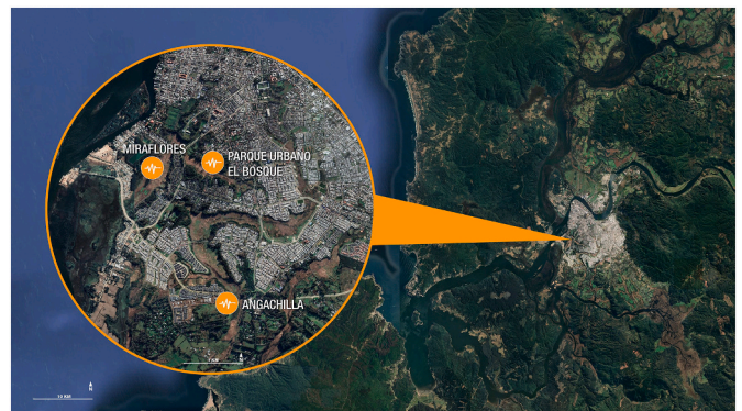
Fig. 1. Map of the three monitoring areas: Angachilla, Miraflores, and Parque Urbano El Bosque in the city of Valdivia, Chile (−39.839, −73.243).
