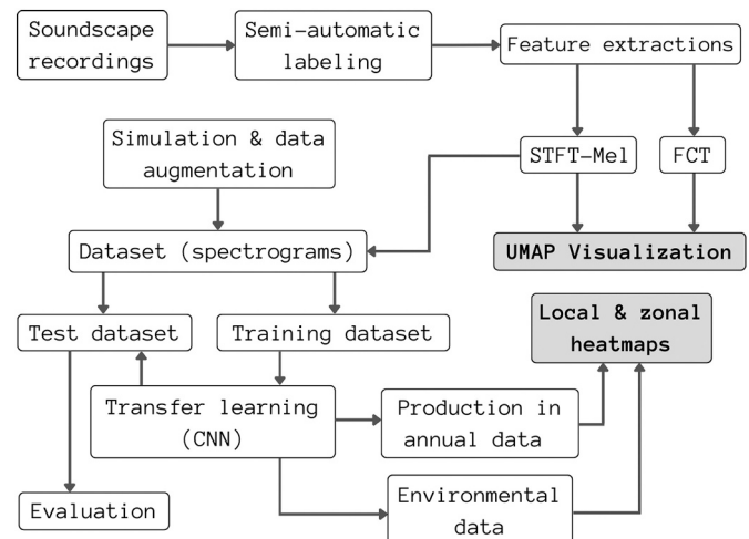
Fig. 3. Workflow diagram of the designed method.
